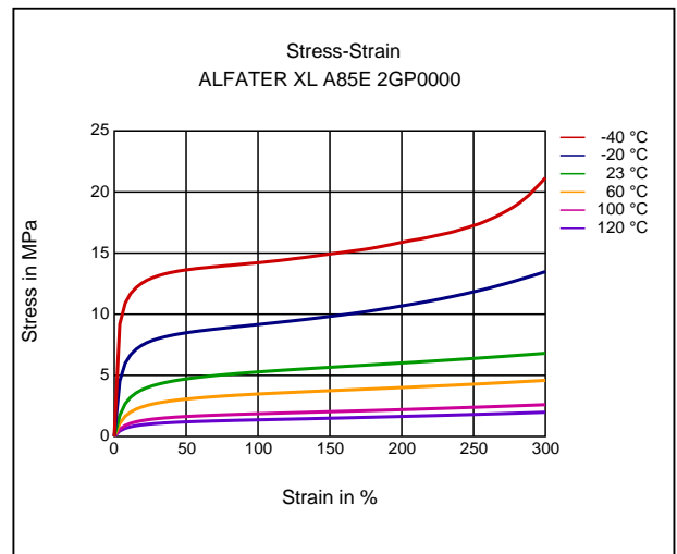
Stress-Strain
